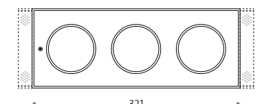
Deckenausschnitt Ceiling cut-out Ø 323×125mm
