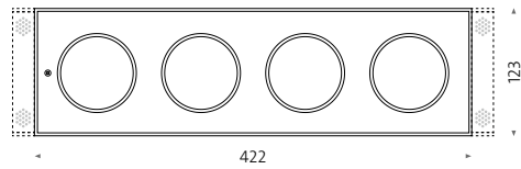
Deckenausschnitt Ceiling cut-out 424x125mm
