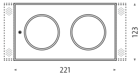
Deckenausschnitt Ceiling cut-out Ø 223×125mm
